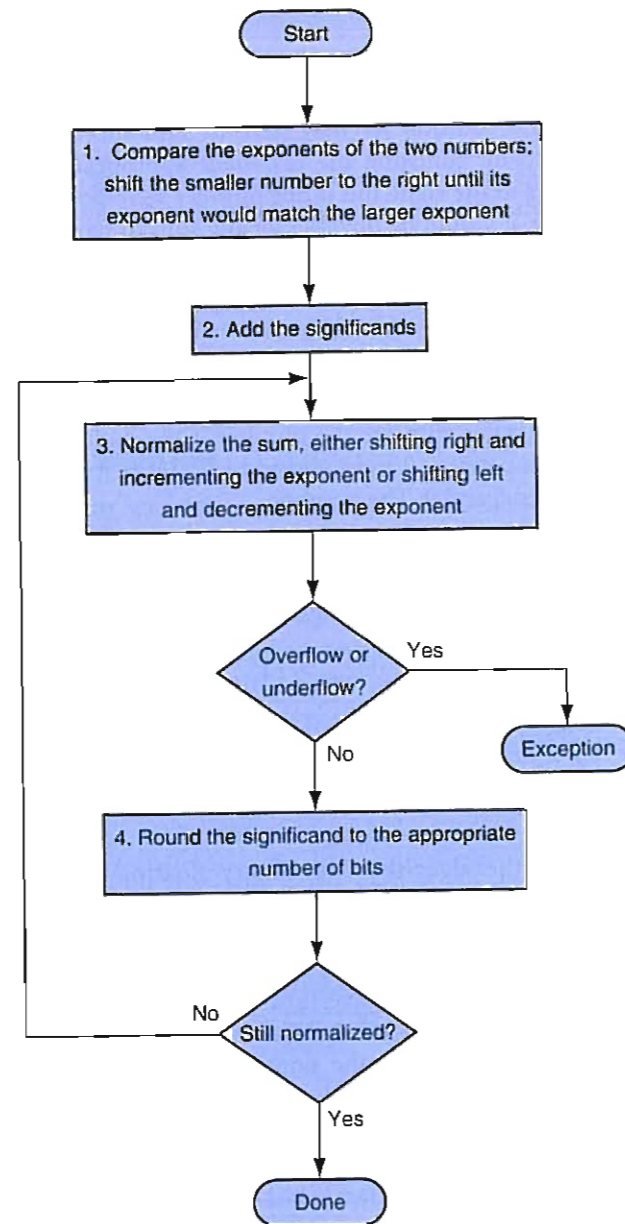
FIGURE 3.15 Floating-point addition. The normal path is to execute steps 3 and 4 once, but if rounding causes the sum to be unnormalized, we must repeat step 3.
