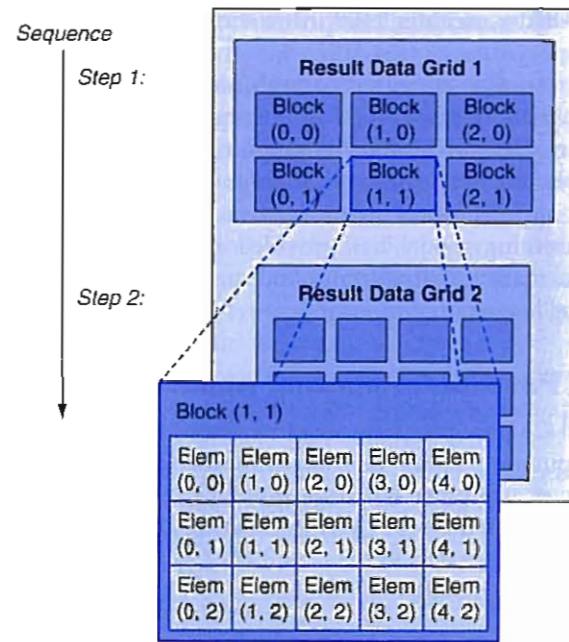
FIGURE A.3.3 Decomposing result data into a grid of blocks of elements to be computed in parallel.
