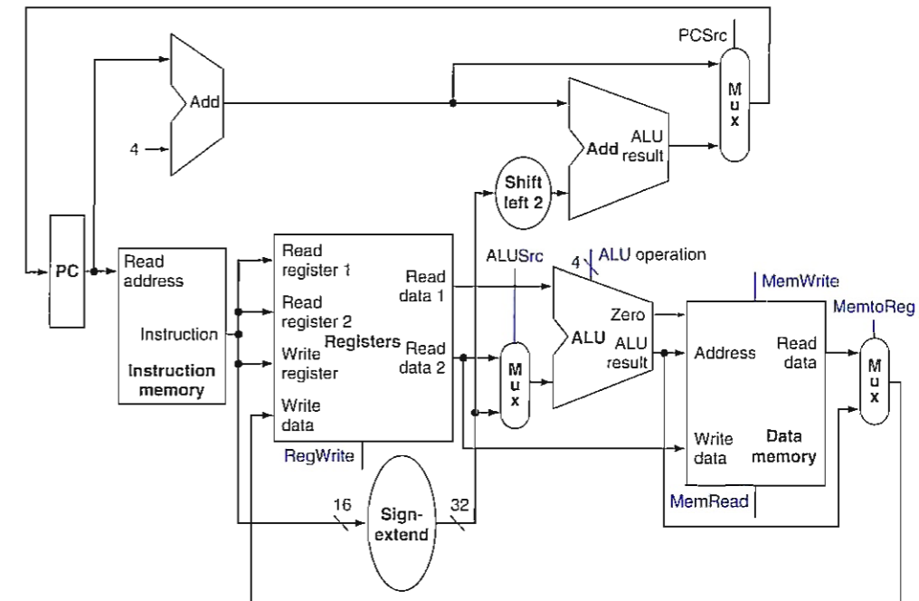
FIGURE 4.11 The simple datapath for the MIPS architecture combines the elements required by different instruction classes. The components come from Figures 4.6, 4.9, and 4.10. This datapath can execute the basic instructions (load-store word, ALU operations, and branches) in a single clock cycle. An additional multiplexor is needed to integrate branches. The support for jumps will be added later.
