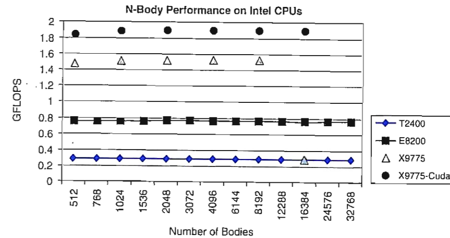
FIGURE A.8.16 Performance measurements on the N-body code on a CPU. The graph shows single precision N -body performance using Intel Core2 CPUs, denoted by their CPU model number. Note the dramatic reduction in GFLOPS performance (shown in GFLOPS on the y -axis), demonstrating how much faster the GPU is compared to the CPU. The performance on the CPU is generally independent of problem size, except for an anomalously low performance when N = 16,384 on the X9775 CPU. The graph also shows the results of running the CUDA version of the code (using the CUDA-for-CPU compiler) on a single CPU core, where it outperforms the C++ code by 24%. As a programming language, CUDA exposes parallelism and locality that a compiler can exploit. The Intel CPUs are a 3.2 GHz Extreme X9775 (code named "Penryn"), a 2.66 GHz E8200 (code named "Wolfdale"), a desktop, pre-Penryn CPU, and a 1.83 GHz T2400 (code named "Yonah"), a 2007 laptop CPU. The Penryn version of the Core 2 architecture is particularly interesting for N -body calculations with its 4-bit divider, allowing division and square root operations to execute four times faster than previous Intel CPUs.
