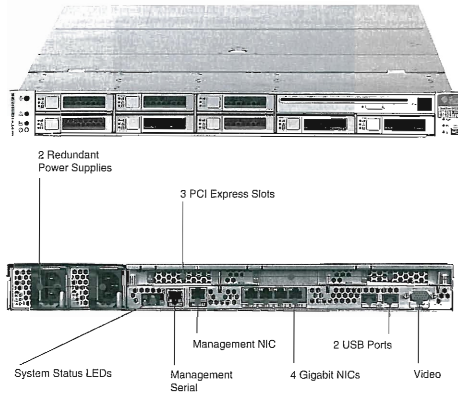
FIGURE 6.16 The front and rear of the Sun Fire x4150 1U server. The dimensions are 1.75 inches high by 19 inches wide. The eight 2.5-inch disk drives can be replaced from the front. In the upper right is a DVD and two USB ports. The picture below labels the items at the rear of the server. It has redundant power supplies and fans to allow the server to continue operating despite failures of one of these components.
