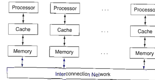
FIGURE 7.4 Classic organization of a multiprocessor with multiple private address spaces, traditionally called a message-passing multiprocessor . Note that unlike the SMP in Figure 7.2, the interconnection network is not between the caches and memory but is instead between processor-memory nodes.
