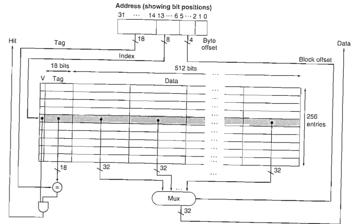
FIGURE 5.9 The 16 KB caches in the Intrinsicity FastMATH each contain 256 blocks with 16 words per block. The tag field is 18 bits wide and the index field is 8 bits wide, while a 4-bit field (bits 5–2) is used to index the block and select the word from the block using a 16-to-1 multiplexor. In practice, to eliminate the multiplexor, caches use a separate large RAM for the data and a smaller RAM for the tags, with the block offset supplying the extra address bits for the large data RAM. In this case, the large RAM is 32 bits wide and must have 16 times as many words as blocks in the cache.
