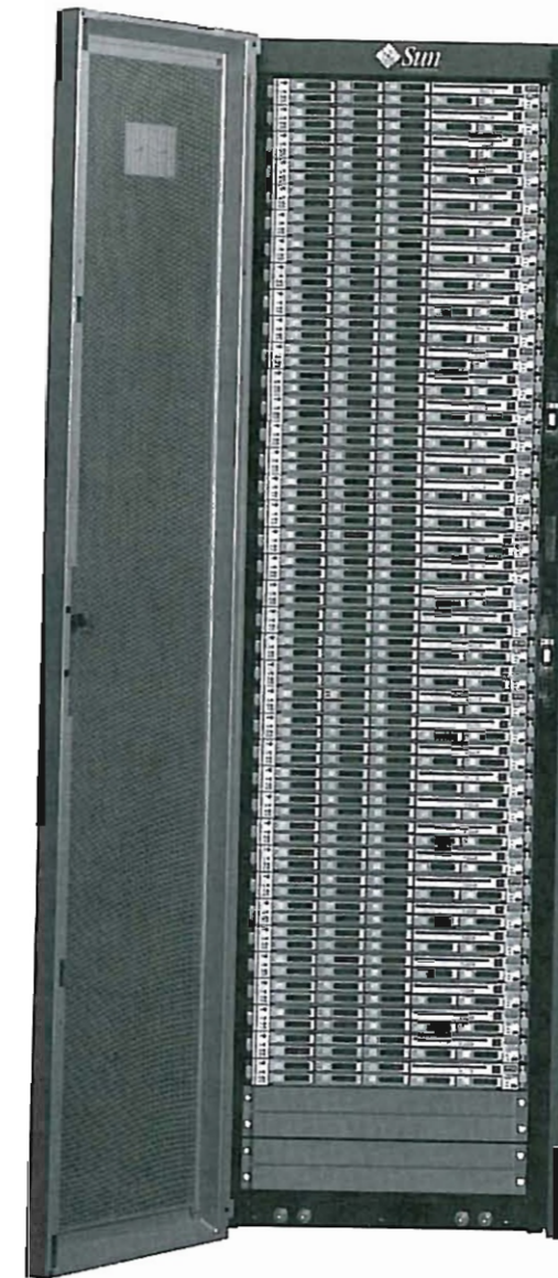
FIGURE 6.15 A standard 19-inch rack populated with 42 1U servers. This rack has 42 1U “pizza box” servers. Source: http://gchelpdesk.ualberta.ca/news/07mar06/cbhd_news_07mar06.php .
