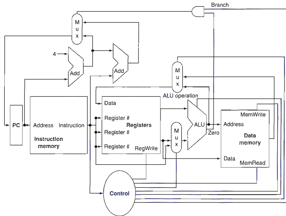
FIGURE 4.2 The basic implementation of the MIPS subset, including the necessary multiplexers and control lines. The top multiplexer (“Mux”) controls what value replaces the PC ( PC + 4 or the branch destination address); the multiplexer is controlled by the gate that “ANDs” together the Zero output of the ALU and a control signal that indicates that the instruction is a branch. The middle multiplexer, whose output returns to the register file, is used to steer the output of the ALU (in the case of an arithmetic-logical instruction) or the output of the data memory (in the case of a load) for writing into the register file. Finally, the bottommost multiplexer is used to determine whether the second ALU input is from the registers (for an arithmetic-logical instruction OR a branch) or from the offset field of the instruction (for a load or store). The added control lines are straightforward and determine the operation performed at the ALU, whether the data memory should read or write, and whether the registers should perform a write operation. The control lines are shown in color to make them easier to see.
