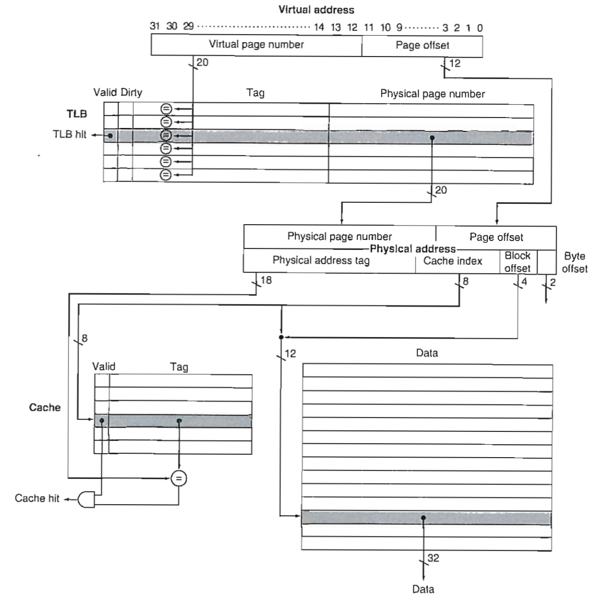
FIGURE 5.24 The TLB and cache implement the process of going from a virtual address to a data item in the Intrinsicity FastMATH. This figure shows the organization of the TLB and the data cache, assuming a 4 KB page size. This diagram focuses on a read; Figure 5.25 describes how to handle writes. Note that unlike Figure 5.9, the tag and data RAMs are split. By addressing the long but narrow data RAM with the cache index concatenated with the block offset, we select the desired word in the block without a 16:1 multiplexor. While the cache is direct mapped, the TLB is fully associative. Implementing a fully associative TLB requires that every TLB tag be compared against the virtual page number, since the entry of interest can be anywhere in the TLB. (See content addressable memories in the Elaboration on page 485.) If the valid bit of the matching entry is on, the access is a TLB hit, and bits from the physical page number together with bits from the page offset form the index that is used to access the cache.
