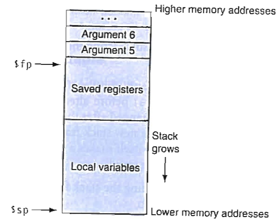
FIGURE B.6.2 Layout of a stack frame. The frame pointer ($fp) points to the first word in the currently executing procedure's stack frame. The stack pointer ($sp) points to the last word of the frame. The first four arguments are passed in registers, so the fifth argument is the first one stored on the stack.
