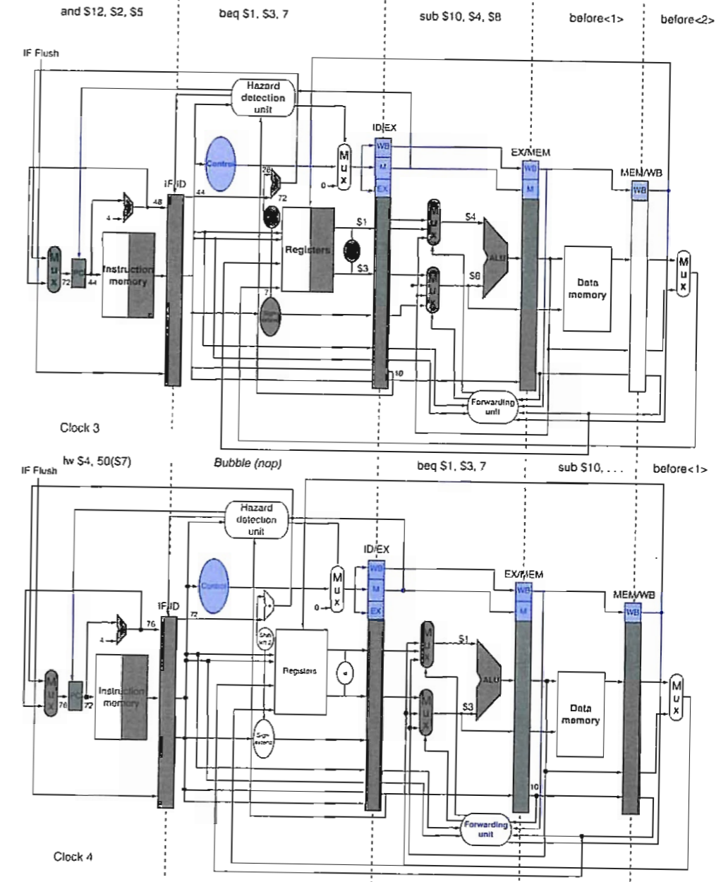
FIGURE 4.62 The ID stage of clock cycle 3 determines that a branch must be taken, so it selects 72 as the next PC address and zeros the instruction fetched for the next cycle. Clock cycle 4 shows the instruction at location 72 being fetched and the single bubble or nop instruction in the pipeline as a result of the taken branch. (Since the nop is really slt $0, $0, 0 , it's arguable whether or not the ID stage in clock 4 should be highlighted.)
