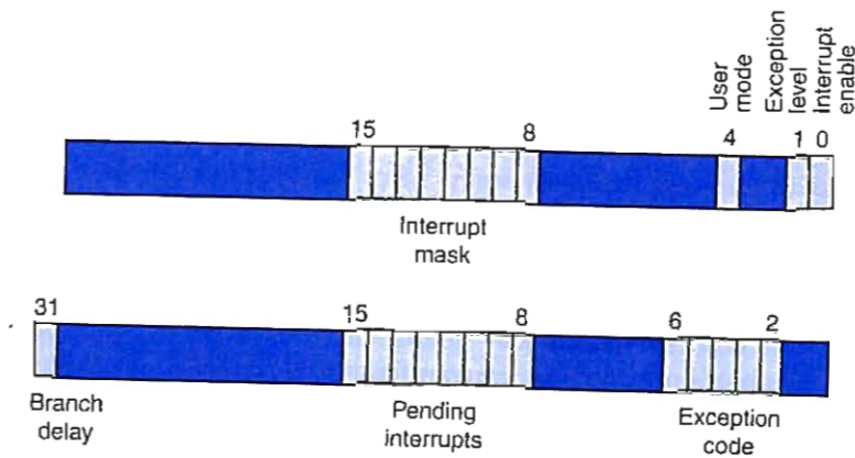
FIGURE 6.11 The Cause and Status registers. This version of the Cause register corresponds to the MIPS-32 architecture. The earlier MIPS 1 architecture had three nested sets of kernel/user and interrupt enable bits to support nested interrupts. Section B.7 in Appendix B has more details about these registers.
