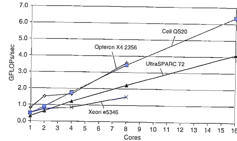
FIGURE 7.20 Performance of SpMV on the four multicores.
