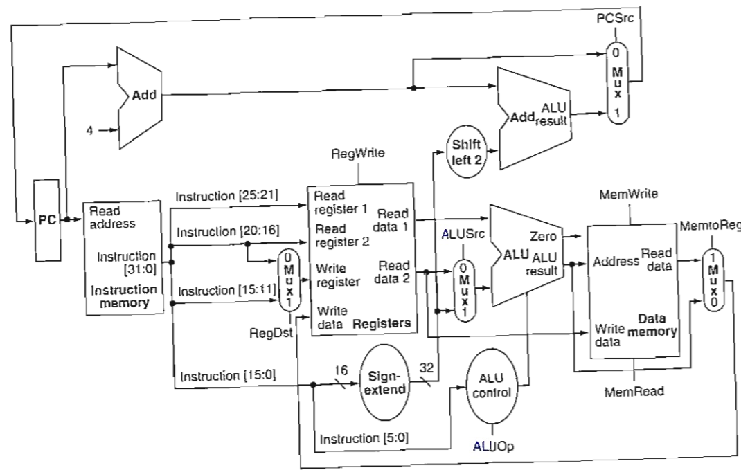
FIGURE 4.15 The datapath of Figure 4.12 with all necessary multiplexers and all control lines identified. The control lines are shown in color. The ALU control block has also been added. The PC does not require a write control, since it is written once at the end of every clock cycle; the branch control logic determines whether it is written with the incremented PC or the branch target address.
