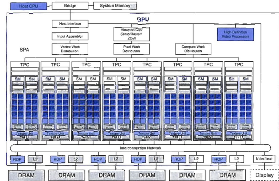
FIGURE A.7.1 NVIDIA Tesla unified graphics and computing GPU architecture. This GeForce 8800 has 128 streaming processor (SP) cores in 16 streaming multiprocessors (SM), arranged in eight texture/processor clusters (TPC). The processors connect with six 64-bit-wide DRAM partitions via an interconnection network. Other GPUs implementing the Tesla architecture vary the number of SP cores, SMs, DRAM partitions, and other units.
