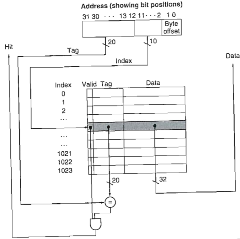
FIGURE 5.7 For this cache, the lower portion of the address is used to select a cache entry consisting of a data word and a tag. This cache holds 1024 words or 4 KB. We assume 32-bit addresses in this chapter. The tag from the cache is compared against the upper portion of the address to determine whether the entry in the cache corresponds to the requested address. Because the cache has 2^{10} (or 1024) words and a block size of one word, 10 bits are used to index the cache, leaving 32 - 10 - 2 = 20 bits to be compared against the tag. If the tag and upper 20 bits of the address are equal and the valid bit is on, then the request hits in the cache, and the word is supplied to the processor. Otherwise, a miss occurs.
