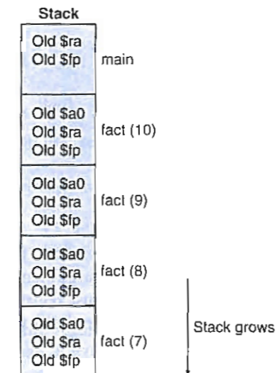
FIGURE B.6.3 Stack frames during the call of fact(7) .
