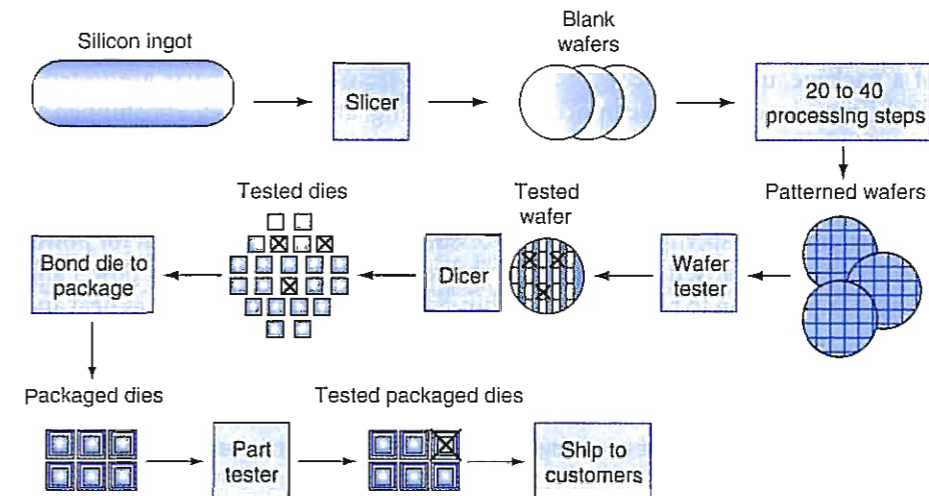
FIGURE 1.18 The chip manufacturing process. After being sliced from the silicon ingot, blank wafers are put through 20 to 40 steps to create patterned wafers (see Figure 1.19). These patterned wafers are then tested with a wafer tester, and a map of the good parts is made. Then, the wafers are diced into dies (see Figure 1.9). In this figure, one wafer produced 20 dies, of which 17 passed testing. (X means the die is bad.) The yield of good dies in this case was 17/20, or 85%. These good dies are then bonded into packages and tested one more time before shipping the packaged parts to customers. One bad packaged part was found in this final test.
