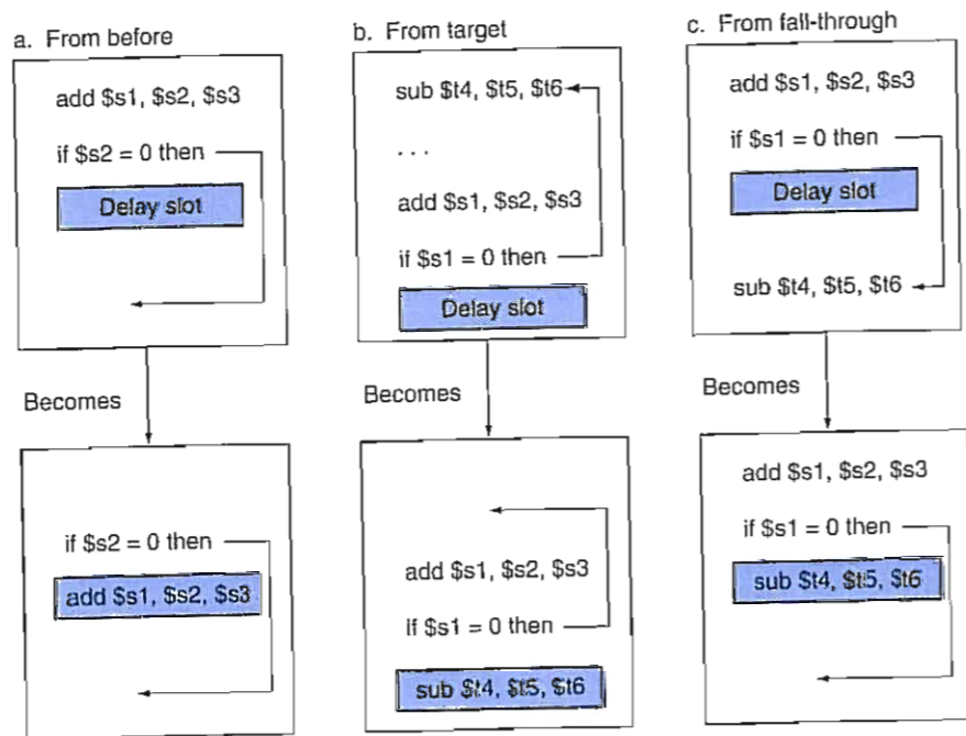
FIGURE 4.64 Scheduling the branch delay slot. The top box in each pair shows the code before scheduling; the bottom box shows the scheduled code. In (a), the delay slot is scheduled with an independent instruction from before the branch. This is the best choice. Strategies (b) and (c) are used when (a) is not possible. In the code sequences for (b) and (c), the use of \$s1 in the branch condition prevents the add instruction (whose destination is \$s1 ) from being moved into the branch delay slot. In (b) the branch delay slot is scheduled from the target of the branch; usually the target instruction will need to be copied because it can be reached by another path. Strategy (b) is preferred when the branch is taken with high probability, such as a loop branch. Finally, the branch may be scheduled from the not-taken fall-through as in (c). To make this optimization legal for (b) or (c), it must be OK to execute the sub instruction when the branch goes in the unexpected direction. By "OK" we mean that the work is wasted, but the program will still execute correctly. This is the case, for example, if \$t4 were an unused temporary register when the branch goes in the unexpected direction.
