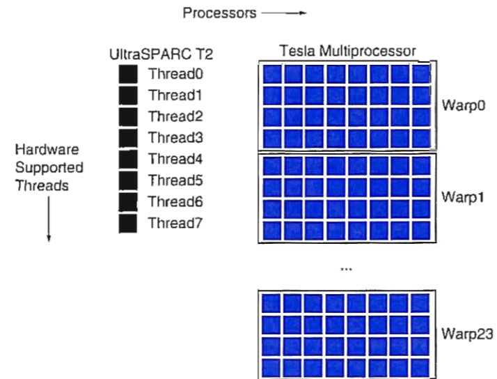
FIGURE 7.7 Comparing single core of a Sun UltraSPARC T2 (Niagara 2) to a single Tesla multiprocessor. The T2 core is a single processor and uses hardware-supported multithreading with eight threads. The Tesla multiprocessor contains eight streaming processors and uses hardware-supported multithreading with 24 warps of 32 threads (eight processors times four clock cycles). The T2 can switch every clock cycle, while the Tesla can switch only every two or four clock cycles. One way to compare the two is that the T2 can only multithread the processor over time, while Tesla can multithread over time and over space; that is, across the eight streaming processors as well as segments of four clock cycles.
