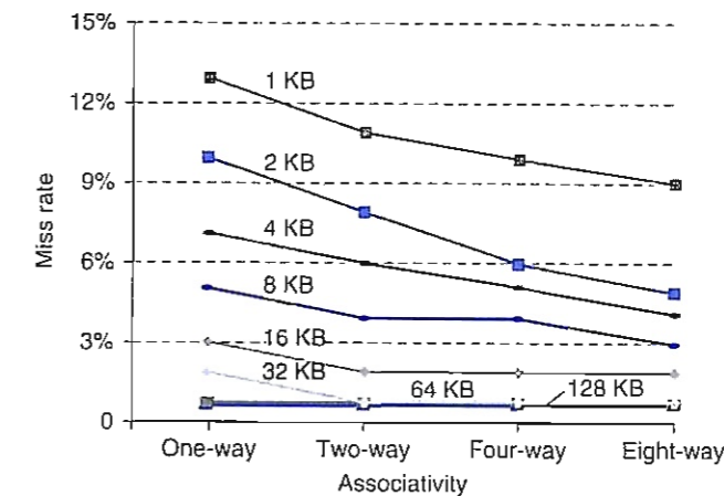
FIGURE 5.30 The data cache miss rates for each of eight cache sizes improve as the associativity increases. While the benefit of going from one-way (direct mapped) to two-way set associative is significant, the benefits of further associativity are smaller (e.g., 1%–10% improvement going from two-way to four-way versus 20%–30% improvement going from one-way to two-way). There is even less improvement in going from four-way to eight-way set associative, which, in turn, comes very close to the miss rates of a fully associative cache. Smaller caches obtain a significantly larger absolute benefit from associativity because the base miss rate of a small cache is larger. Figure 5.15 explains how this data was collected.
