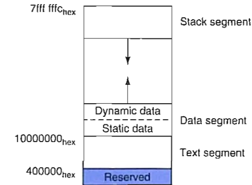
FIGURE B.5.1 Layout of memory.
