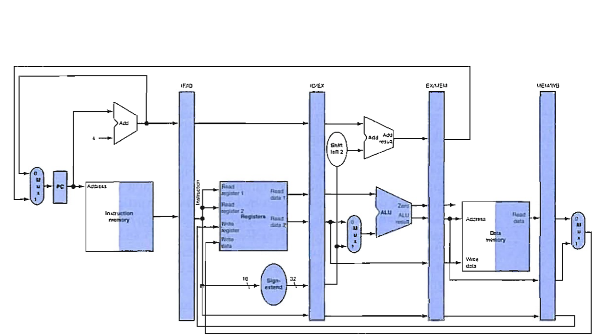
FIGURE 4.42 The portion of the datapath in Figure 4.41 that is used in all five stages of a load instruction.
