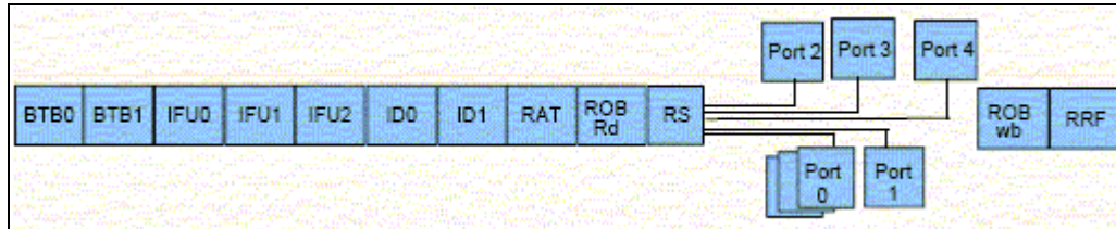
Figure 5.1. Pentium Pro pipeline.
